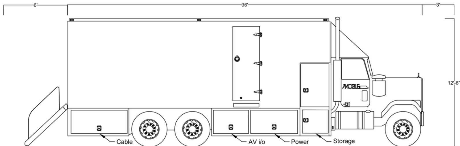
SIDE VIEW (SETUP)
